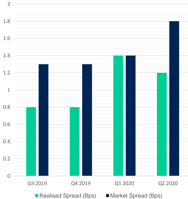
G10 Forwards
