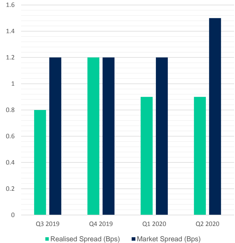
G10 Spot
